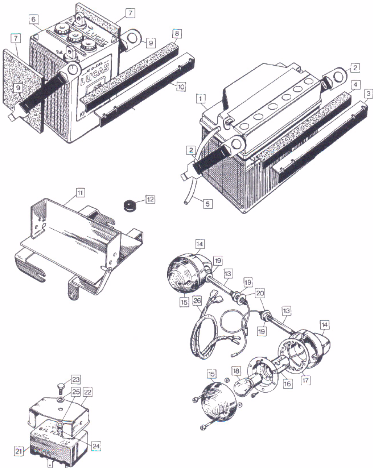
Batteries, Battery Tray, Direction Indicators
