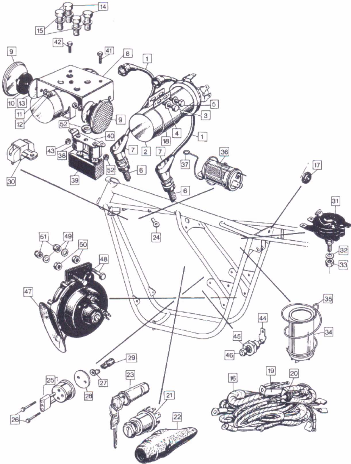
Basic Electrical Components
