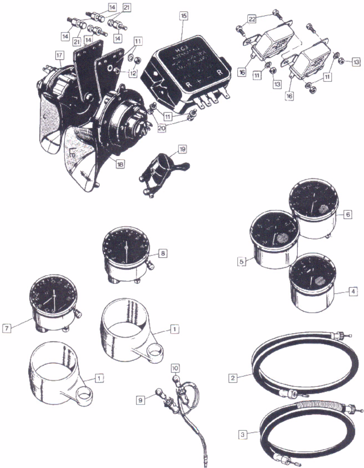
Instruments and Police Horns
