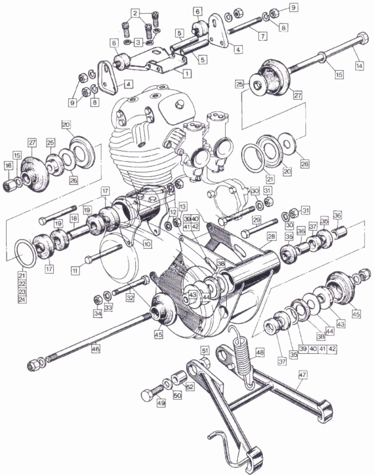
Engine Mountings, Head Steady, Centre Stand
