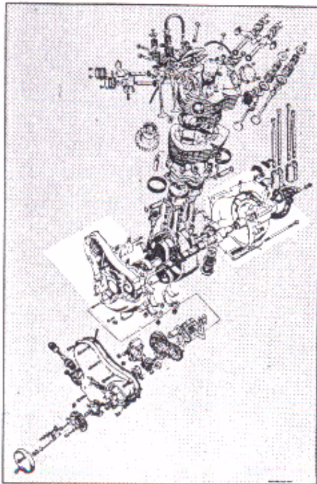
Engine: Crankcases, Crankcase Breather, Tachometer Drive
