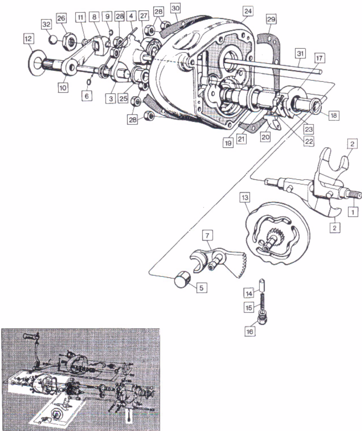
Gearbox: Inner Cover
