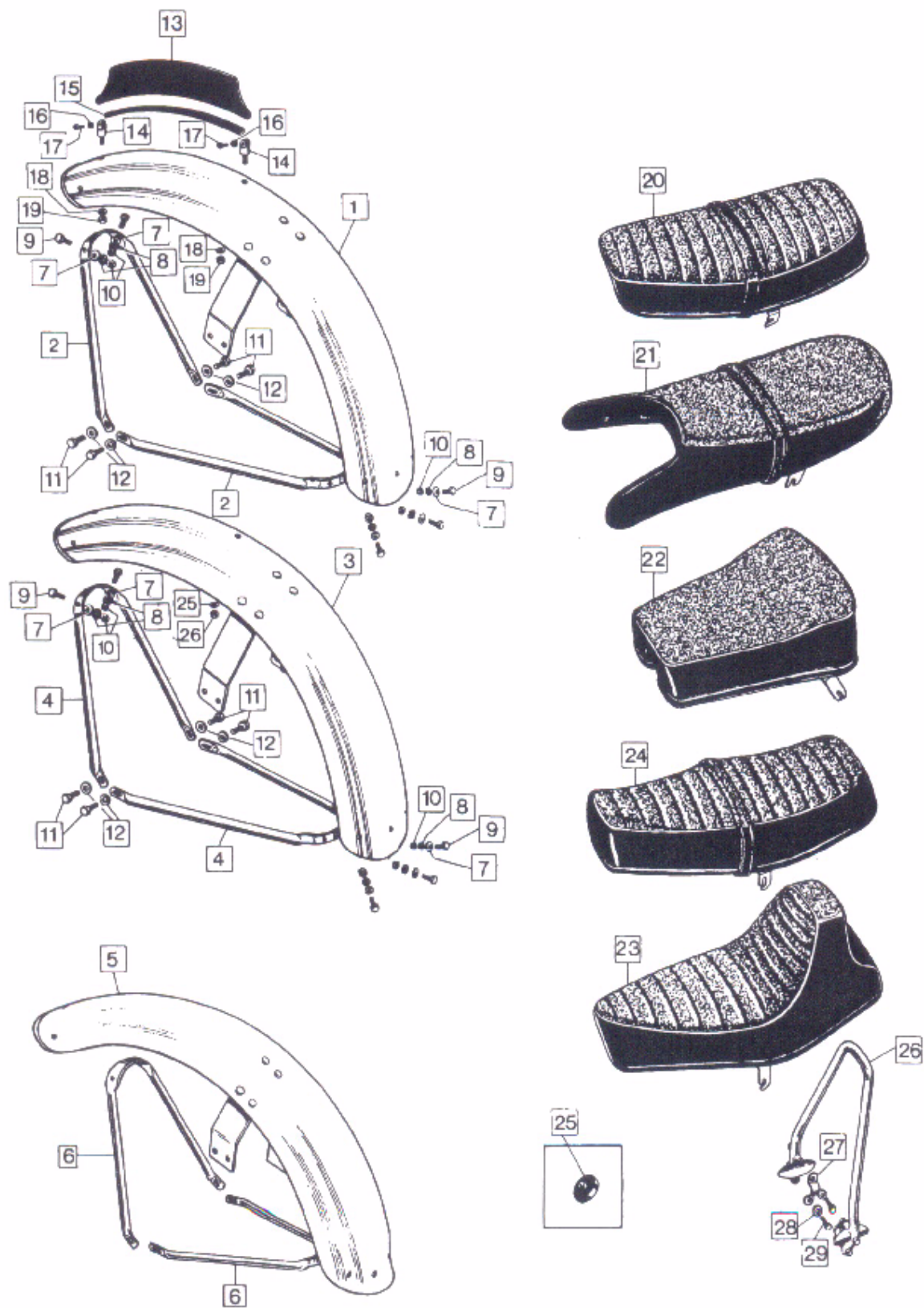
Front Fenders, Number Plate and Seats
